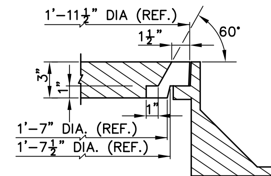
SECTION AT SLOT
