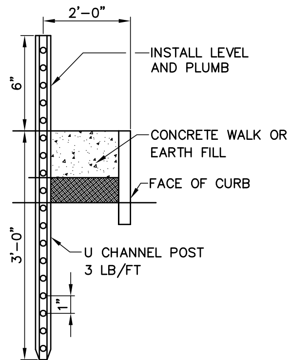
U-CHANNEL POST DETAIL BASE DETAIL N.T.S.
