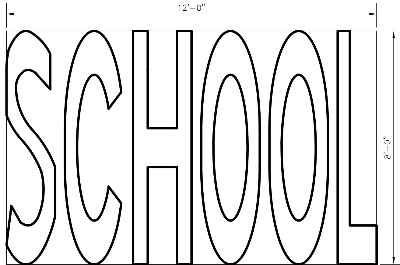
SINGLE-LANE PAVEMENT MARKING DETAIL OF THE WORD "SCHOOL"
