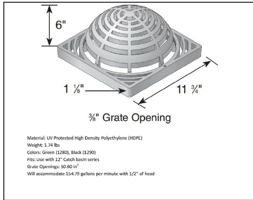
12" x 12" DOME GRATE NOT TO SCALE
